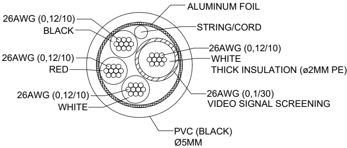
CABLE BUILDUP
