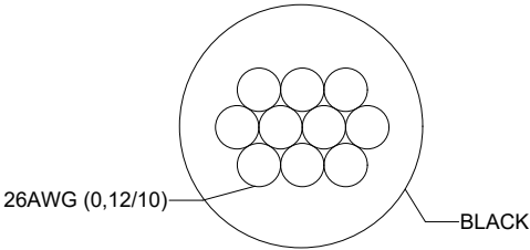
WIRE BUILDUP
