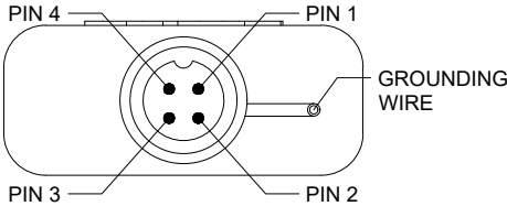
4 PIN MALE MATING FACE
