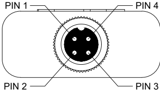
4 PIN FEMALE MATING FACE
